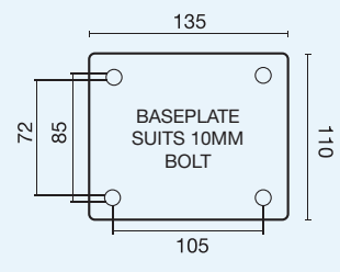
Baseplate for 150-200mm Swivel Castors
