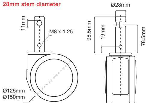
ABS Twin Wheel castors with 28mm stem diameter
