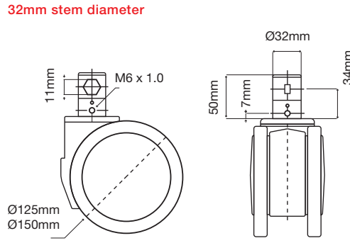
ABS Twin Wheel castors with 32mm stem diameter
