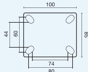
Baseplate for 100-125mm Swivel Castors
