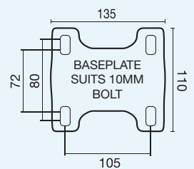
Baseplate for 150-200mm Rigid Castors
