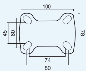
Baseplate for 100-125mm Rigid Castors
