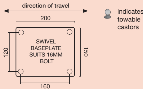
Standard baseplate dimensions and drilling patterns for EHP castors
