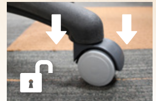
When weight is placed on the castor the brake will release.
