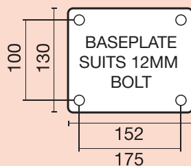
Standard High Performance Series baseplate
